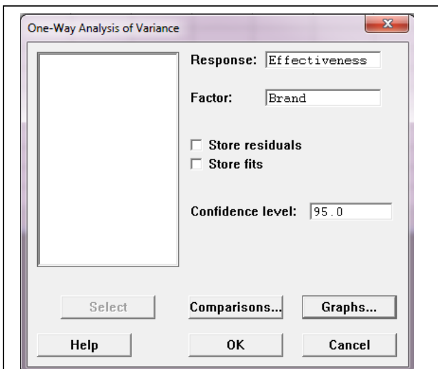
Figure 3b: Selecting Variables in One-WAY ANOVA in MINITAB
